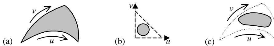
Fig. 4: (a) un-trimmed surface, (b) trimming curve in the parameter domain, and (c) trimmed surface.
