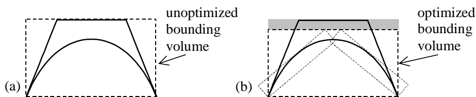
Fig. 9: (a) un-optimized and (b) optimized bounding volume.
