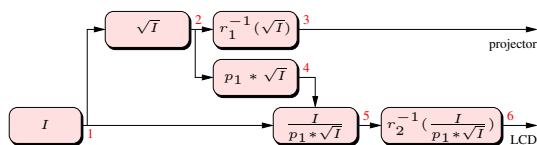
Figure 5: Rendering algorithm for the projector-based display.
