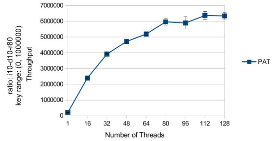
Figure 10. Replace operations of PAT
