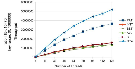
Figure 11. Non-uniformly distributed keys (The lines for 4-ST, BST, AVL and SL overlap.)
