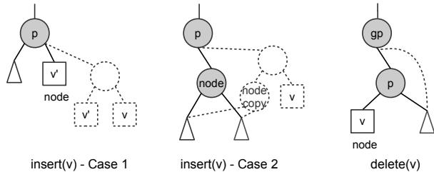
Figure 5. Different cases of \text{insert}(v) and \text{delete}(v) . Triangles are either a leaf node or a subtree. The grey circles are flagged nodes. The dotted lines are the new child pointers that replace the old child pointers (solid lines) and the dotted circles and squares are newly created nodes.
