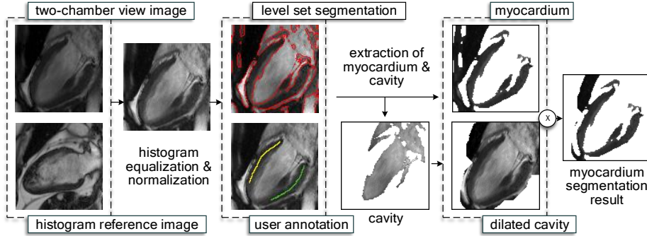
Fig. 1. Steps taken before and after applying the multiphase level set segmentation algorithm on the user-annotated two-chamber view image of the LV.
