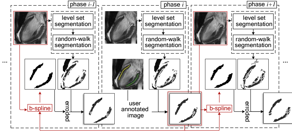
Fig. 3. The segmentation result for the user-annotated ( i th) phase is registered to the (i+1) th phase ( (i-1) th phase) and used as a mask to select segments from the segmentation result for that phase. The registered mask in the (i+1) th phase ( (i-1) th phase) is then registered to the (i+2) nd phase ( (i-1) nd phase) and so on.
