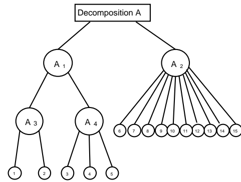
(a) A nested decomposition of a software system
