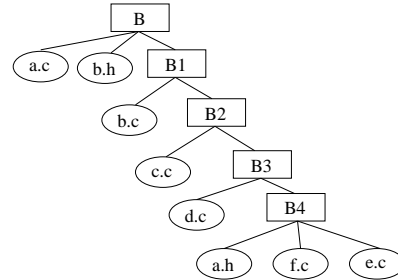
Figure 19. B - Nested Decomposition .
