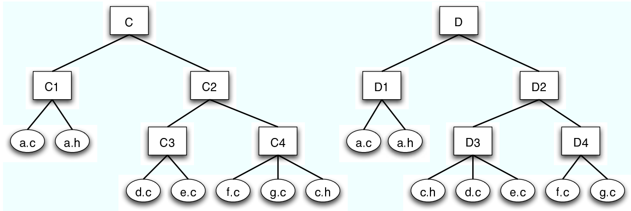
Figure 4. Decompositions C and D
