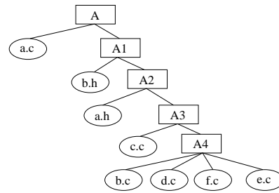
Figure 18. A - Nested Decomposition .
