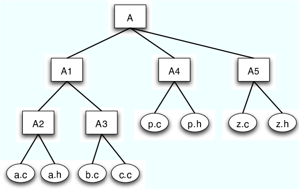
Figure 6. The containment tree of an automatic decomposition A.
