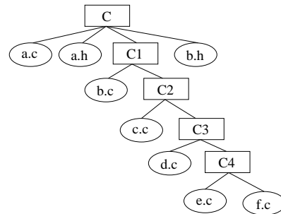
Figure 20. C - Nested Decomposition .
