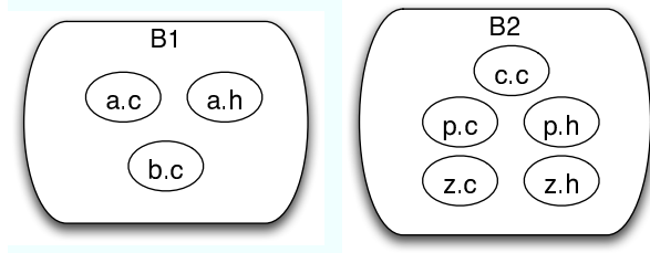
Figure 9. The flat decomposition of nested decomposition B.
