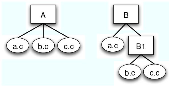
Figure 15. An example of an implicit Down operation
