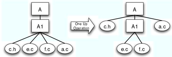
Figure 14. Example of 1 Up operation
