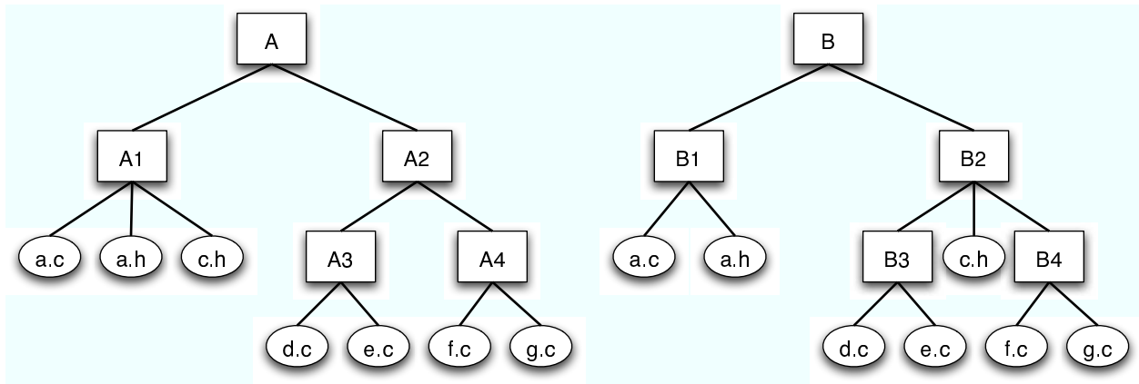
Figure 3. Decompositions A and B
