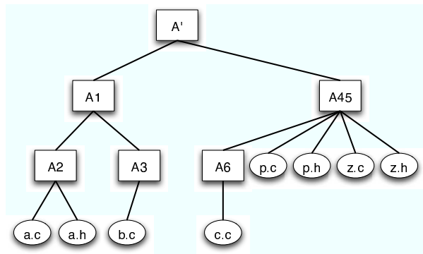
Figure 10. Decomposition A after the transformation indicated by MoJo.
