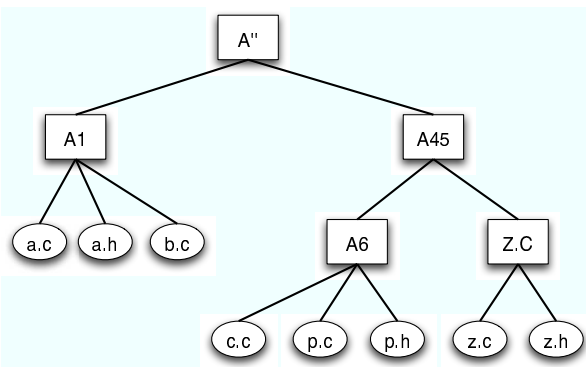
Figure 13. The final containment tree for decomposition A.
