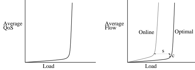
Figure 1: (a) Standard performance curve, and (b) The worst possible performance curve of an s -speed c -competitive online algorithm.
