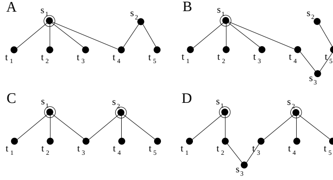
Figure 1: Examples of spanning trees that might be in the queue. A node is circled if it is closed.
