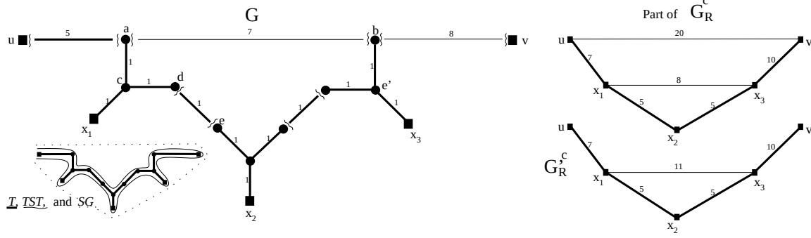
Figure 5: An instance G . The key edges in the metric completion G_R^c with its minimum spanning tree in bold is used to demonstrate the 2-approximate minimal Steiner tree algorithm. The resulting Steiner tree in G (which is optimal) consists of the bold edges plus \{b, v\} . T , TST , and SG used in the proof of correctness of this algorithm is also given. The graph G is partitioned into N(u) and G_R^c with its minimum spanning tree in bold is given as done in the Mehlhorn algorithm. The edges bold in G are those pushed on the stack by our algorithm when \ell = 10 just before the edge \{a, b\} is considered. It is used to demonstrate the proof of correctness of our algorithm.
