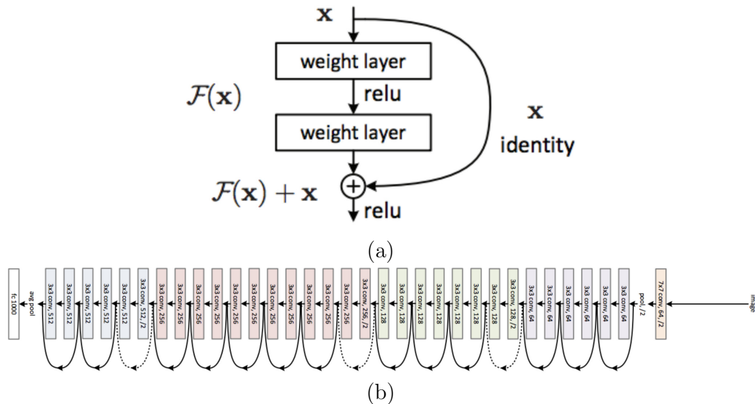
Figure 2.10: ResNet architecture. (a) A residual module. (b) Illustration of a typical ResNet architecture that consists of stacking many residual modules. Figure reproduced from [64].
