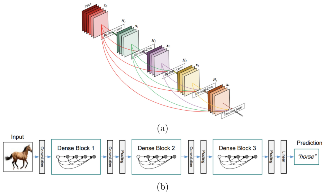
Figure 2.11: DenseNet architecture. (a) A dense module. (b) Illustration of a typical DenseNet architecture that consists of stacking many dense modules. Figure reproduced from [72].
