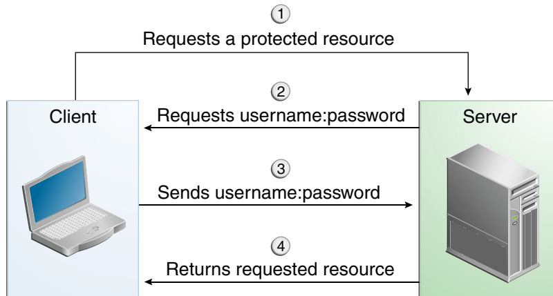
FIGURE 25–2 HTTP Basic Authentication
