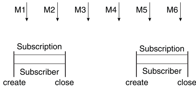
FIGURE 30–6 Nondurable Subscribers and Subscriptions
