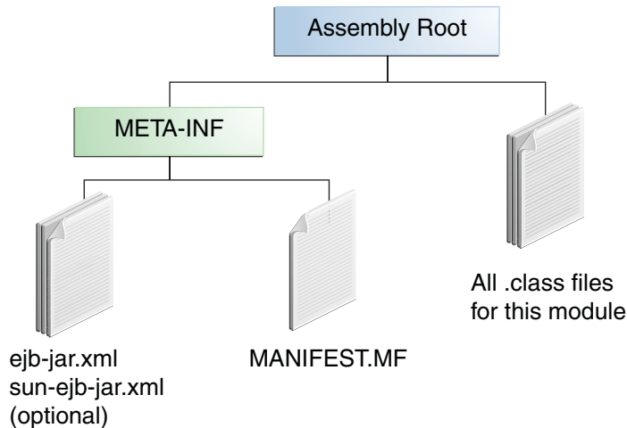
FIGURE 14-2 Structure of an Enterprise Bean JAR
