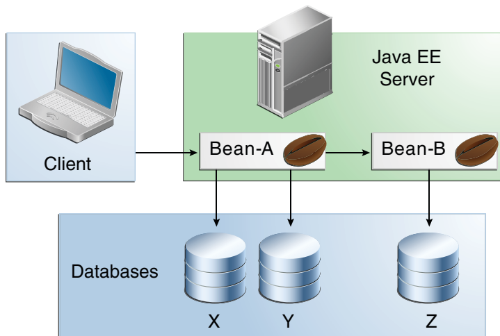
FIGURE 28–2 Updating Multiple Databases
