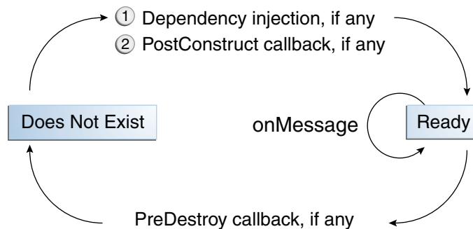
FIGURE 30–9 Lifecycle of a Message-Driven Bean
