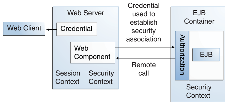
FIGURE 24-5 Invoking an Enterprise Bean Business Method
