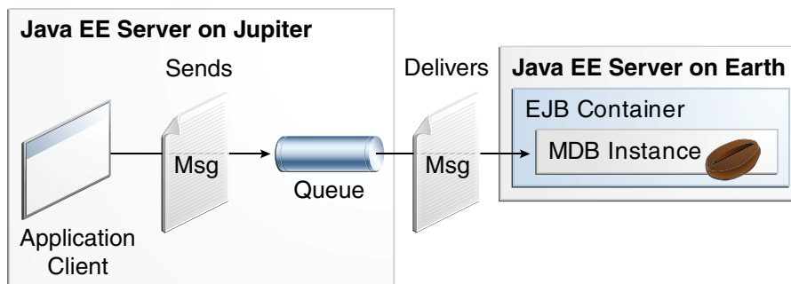
FIGURE 31-5 A Java EE Application That Consumes Messages from a Remote Server
