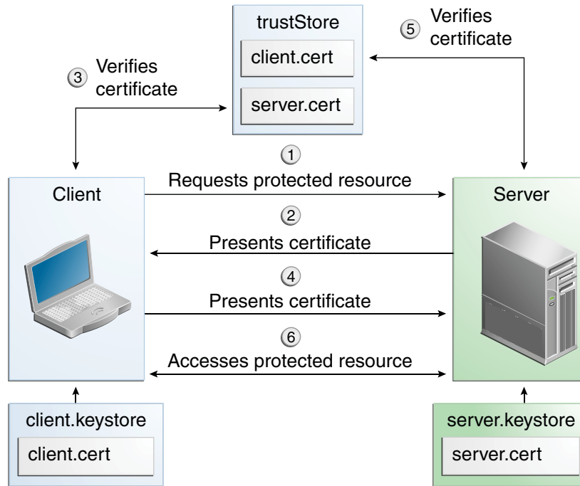
FIGURE 25-4 Certificate-Based Mutual Authentication
