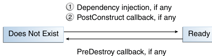
FIGURE 14-4 Lifecycle of a Stateless Session Bean
