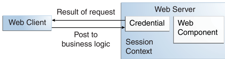
FIGURE 24-4 Fulfilling the Original Request
