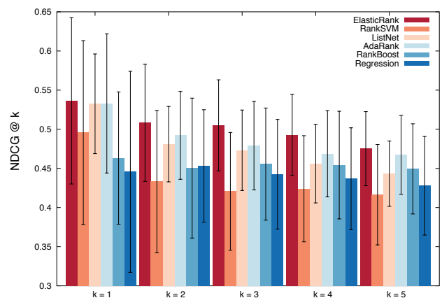
(c) OHSUMED
