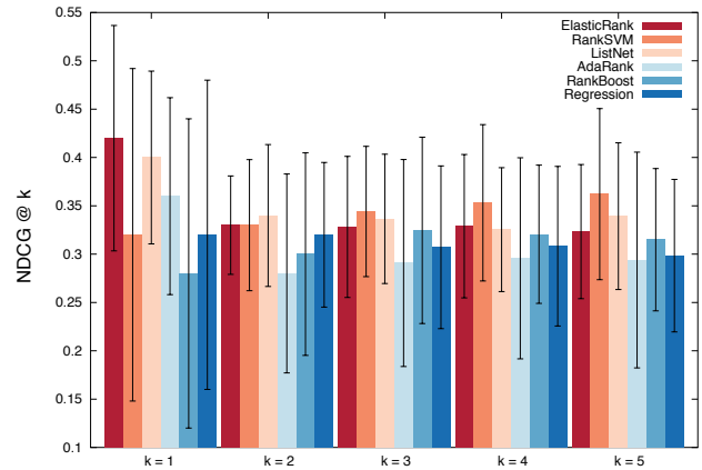
(a) TD2003
