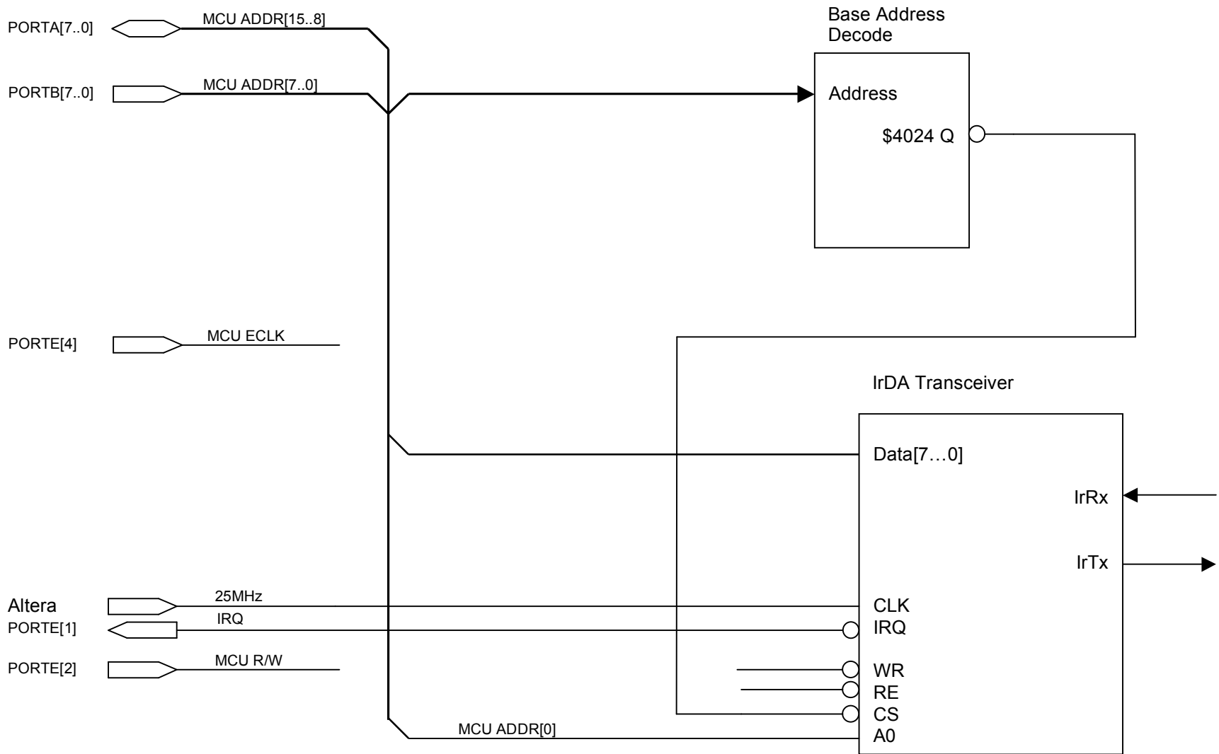
Figure 7.4 IrDA Transceiver HCS12 Extended Narrow Mode Interface
