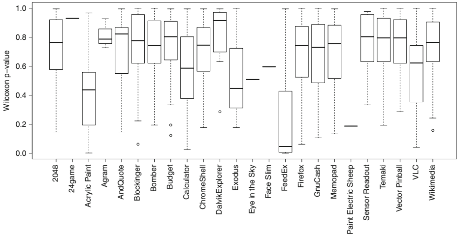
Fig. 3 Wilcoxon Rank Sum p -values per application of energy consumed with logging and without logging. p -values less than 0.05 indicate that logging enabled and logging disabled consumed different amounts of energy. p -values were corrected for multiple hypotheses using Benjamini and Hochberg correction (Benjamini and Hochberg 1995)
