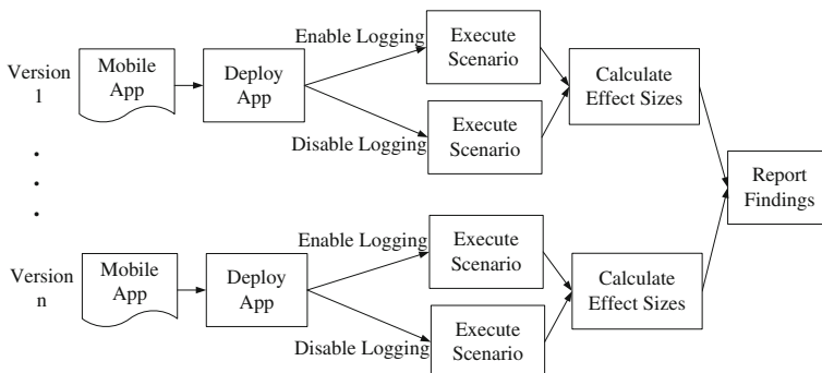
Fig. 2 Process to investigate the energy impact of logging (RQ1)
