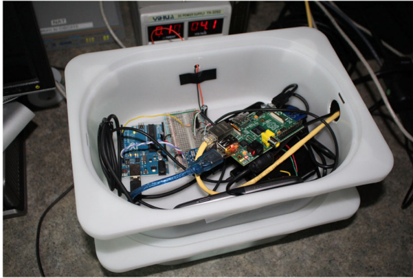
Fig. 1 GreenMiner consists of an Arduino, a breadboard with INA219 chip, a Raspberry Pi, a USB hub, and a Galaxy Nexus phone connected to a Power Supply. Photo used with permission from the Green Miner paper (Hindle et al. 2014)
