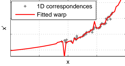
Figure 2. Results from Moving DLT without regularisation for a 1D projective estimation problem on synthetic data.
