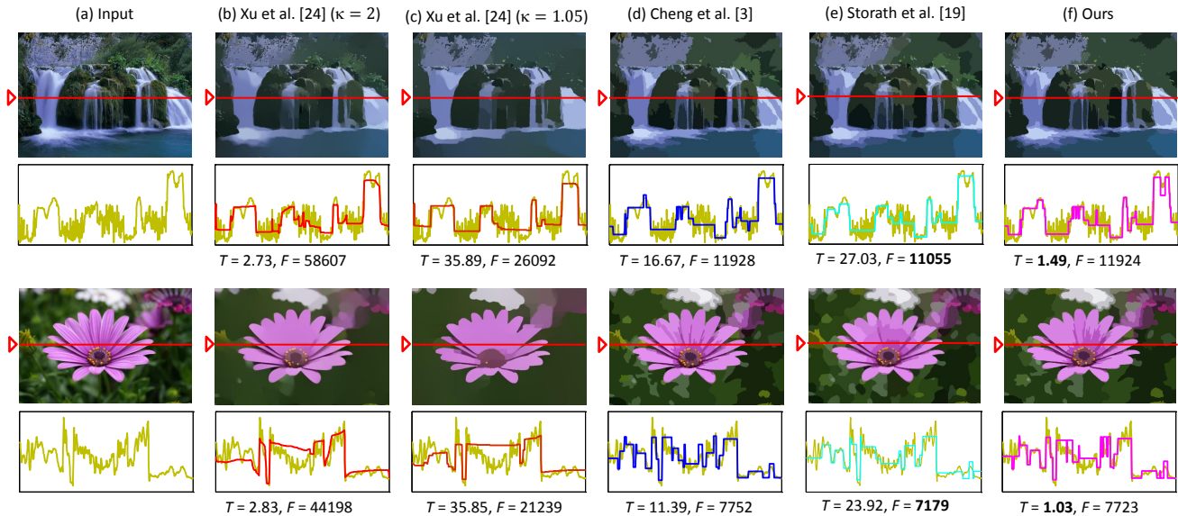
Figure 5. This figure shows the details of the experiment that was already shown in Fig. 1 in Sec. 1. One more result for Xu et al.’s method with \kappa = 2 is added in here. (a) Input images. (b)-(c) Results of Xu et al. [24] with different \kappa = 2 , and \kappa = 1.05 ( \lambda = 0.05 ). (d) Results of Cheng et al. [3] ( \lambda = 0.2 ). (e) Results of Storath et al. [19] ( \lambda = 0.2 ). (f) Our results ( \lambda = 0.2 ). The plot in the second row shows a 1D scanline from the green channel. We also report the running time (in seconds) and the objective function value defined in Equation 2.
