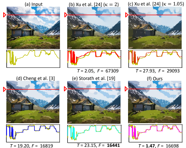
Figure 1. This figure shows the results of applying L_0 gradient minimization on an image by Xu et al. [24], Cheng et al. [3], Storath et al. [19], and our method. Parameters for each method was tuned to produce the best results (closest result to L_0 ). The plots under each image show a 1D scanline from the green channel. We also report the running time T (in seconds) and the final objective function value F (defined in Equation 2) which includes the L_0 regularization.
