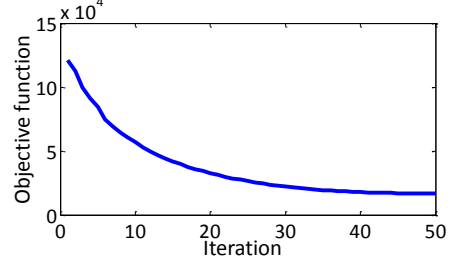
Figure 3. This plot shows the value of the objective function in Equation 2 for each iteration. The input signal is the image shown in Figure 1. The objective function monotonically decreases at each iteration.
