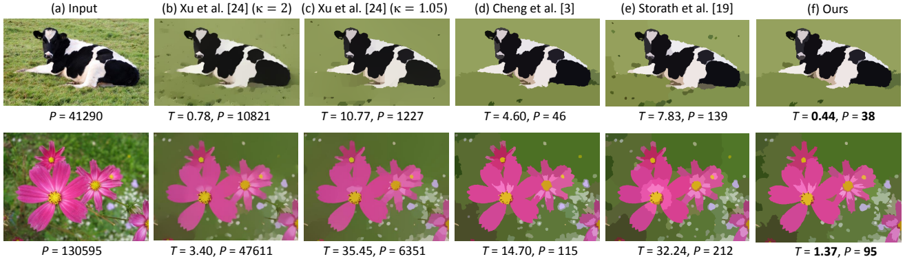
Figure 8. This figure shows several examples of content-based color quantization on images. This is useful for computer vision tasks such as image segmentation or image retrieval. (a) Input images. (b)-(c) Results of Xu et al.’s method with different \kappa = 2 and \kappa = 1.05 . (d) Result of Cheng et al.’s method. (e) Results of Storath et al.’s method. (f) Our results. We also report the running time T (in seconds) and the number of remaining colors P .
