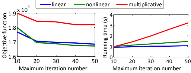
Figure 4. This figure shows the results with different values of the maximum iteration number (e.g. 10, 20, 30, 40, 50) on three strategies for increasing \beta , i.e. linear, nonlinear, and multiplicative. The left shows the values for objective function, F , while the corresponding running-time are shown in the right.
